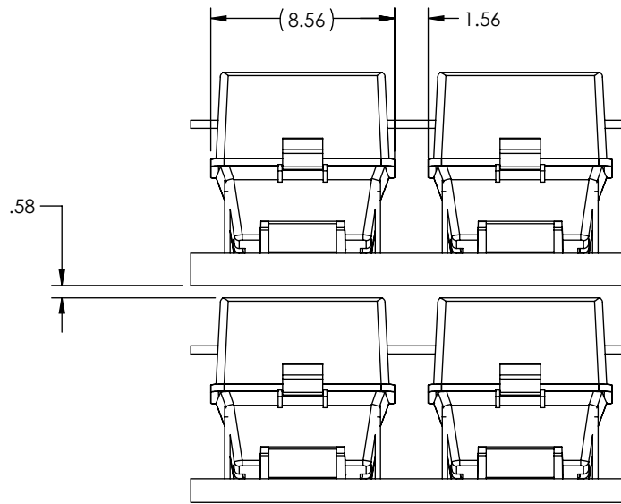
DETAIL D SCALE 1 : 8
